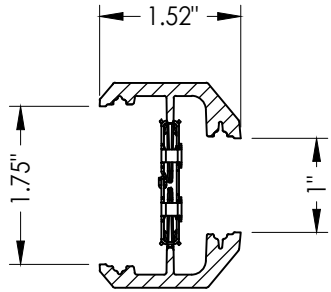
2A ZEEL LITE FRAME CLIP ASSEMBLED FRAME PC/ABS
